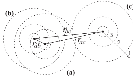
FIG. 1. A sketch of the model. The sketch is for the case of three particles (a, b, and c) with velocity fields composed by three eddies (1, 2, and 3, that corresponds to the three circles of diameter, respectively, l_1 , l_2 , and l_3 ). Tracers positions are indicated by black dots, while dashed circles are correlation radii relative to the eddies with diameter l_1 , l_2 , and l_3 (corresponding to shells 1, 2, and 3). The largest eddy described by the sub-grid-scale model may correspond to the smallest resolved eddy of the Eulerian Large-eddy simulation. In case of a purely Lagrangian evolution, i.e., without a large-scale model or a LES, the largest eddy corresponds to the integral scales of the system, L_0 . The three modes of the velocity of particle “a” are computed by modulating the OU processes associated to particle “a”— \zeta_i^{(a)} with i = 1, 2, 3 —and the OU processes attached to particles “b” and “c”. This is done, in this simple example, according to: \mathbf{v}_1^{(a)} = \zeta_1^{(a)} + \zeta_1^{(b)}(1 - \frac{r_{ab}}{l_1}) + \zeta_1^{(c)}(1 - \frac{r_{ac}}{l_1}) ; \mathbf{v}_2^{(a)} = \zeta_2^{(a)} + \zeta_2^{(b)}(1 - \frac{r_{ab}}{l_2}) ; \mathbf{v}_3^{(a)} = \zeta_3^{(a)} , where we have kept into account the fact that (a) and (b) overlap with shells 1 and 2, while (a) and (c) overlap only with shell 1.
