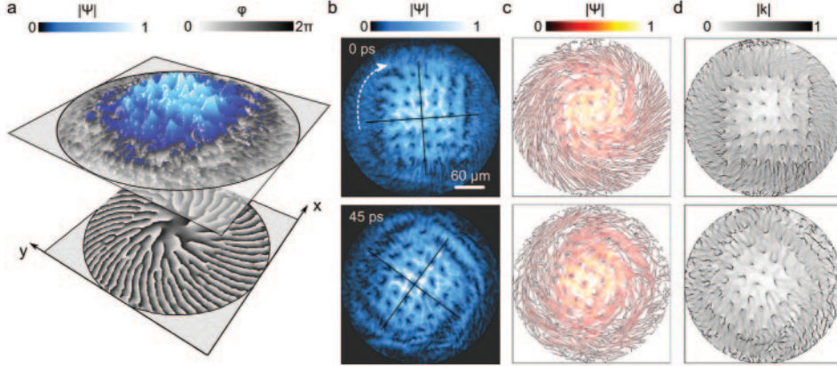
Fig. 1. – Rotating polariton lattice of n^2 = 49 equal charge vortices. (a) The macroscopic wave function amplitude field \psi(\mathbf{x}) on top of the corresponding phase field \varphi(\mathbf{x}) , showing the singularity lattice. (b) Normalized amplitude of \psi(\mathbf{x}, t) at two different times, showing the rigid-like rotation of the system. (c), (d) Direction streamlines and normalized intensity maps of the momentum field, underlying the dynamics.
